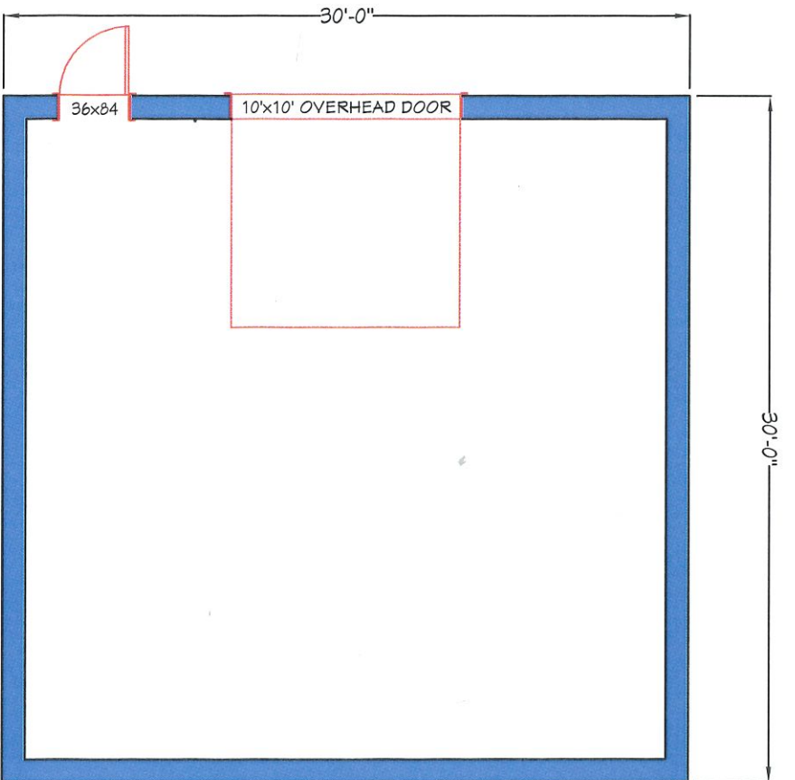
30X30 FLOOR PLAN 900 sq ft
