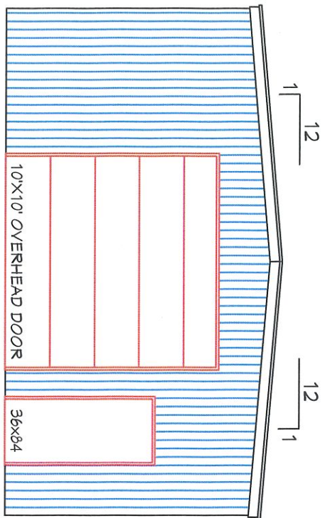
ENDWALL ELEVATION
