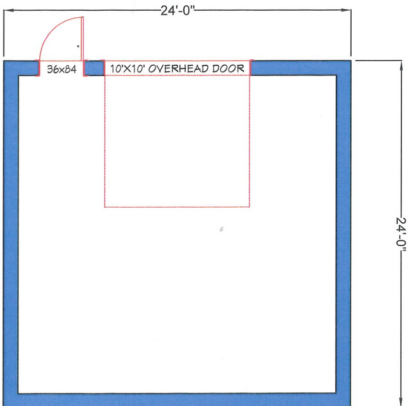
SHOP/GARAGE 576 sq ft
