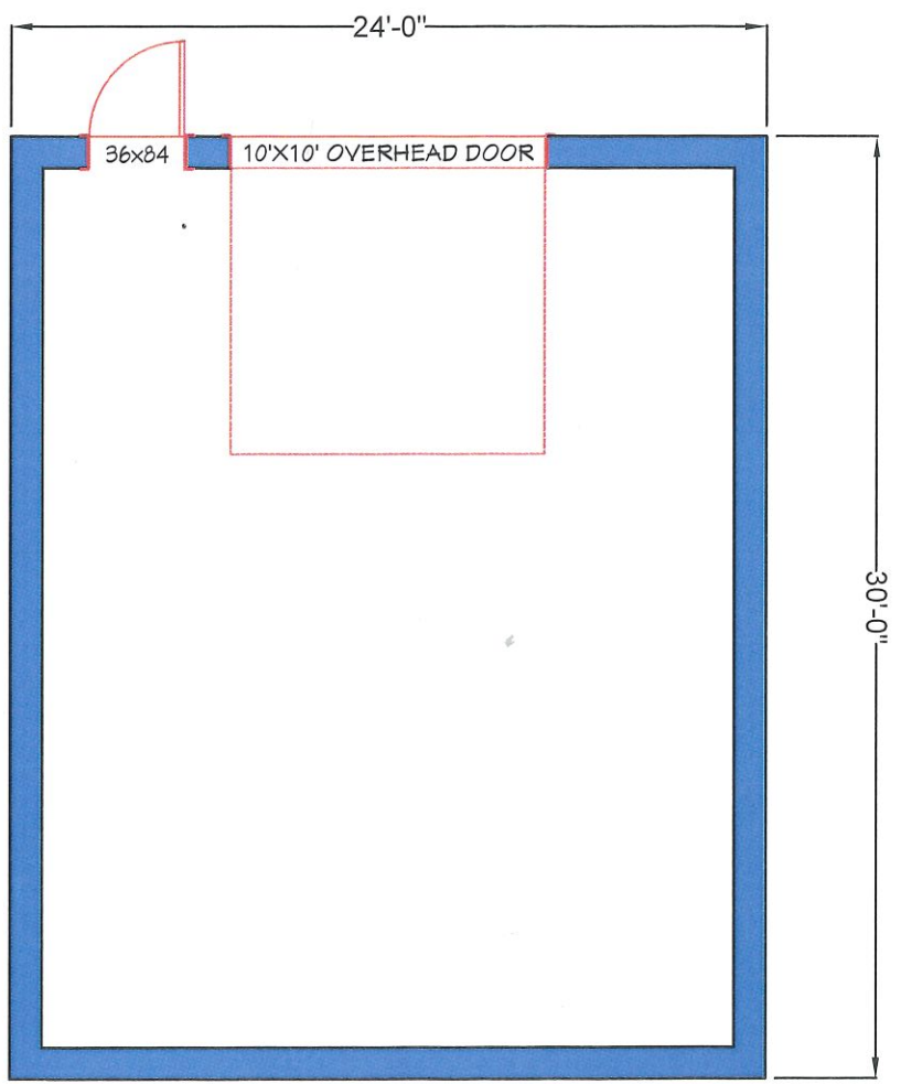
24x30 FLOOR PLAN 720 sq ft
