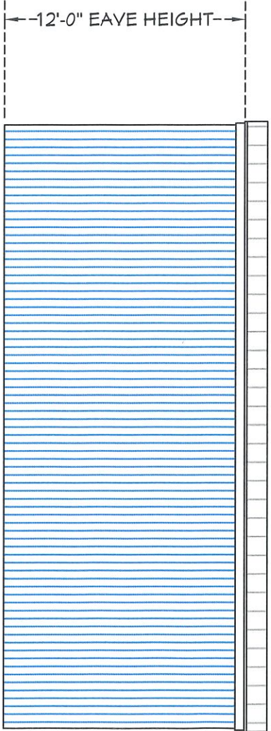
SIDEWALL ELEVATION
