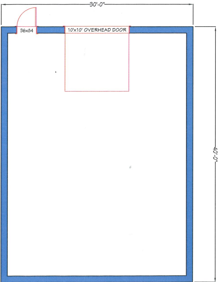
30x40 FLOOR PLAN 1200 sq ft
