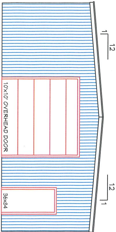
ENDWALL ELEVATION
